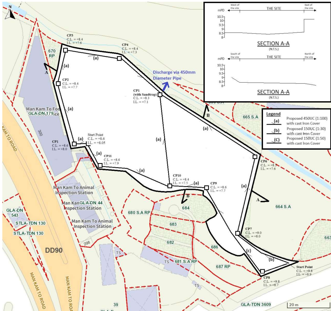
Figure 5 Connection Detail
